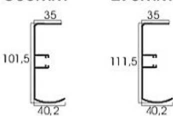
Guia Especial I C80mm Z90mm
